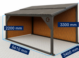
Solar Carport Classic Single 3,9 kW
