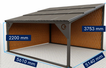
Solar Carport Classic Duo 5,85 kW
