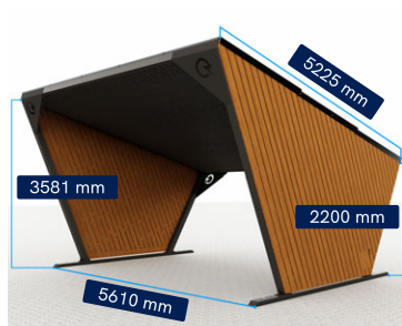
Solar Carport Modern 5,85 kW
